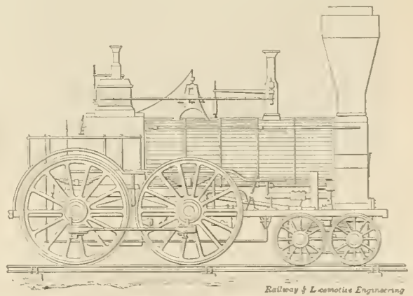
HINKLEY & DRURY ABOUT 1849.
